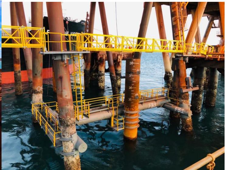
Spud pile bracing and modular access along a long wharf
