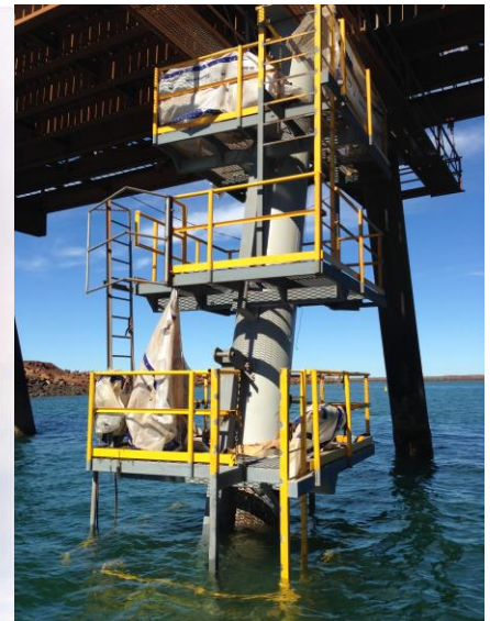
Twin level pile painting horseshoe
