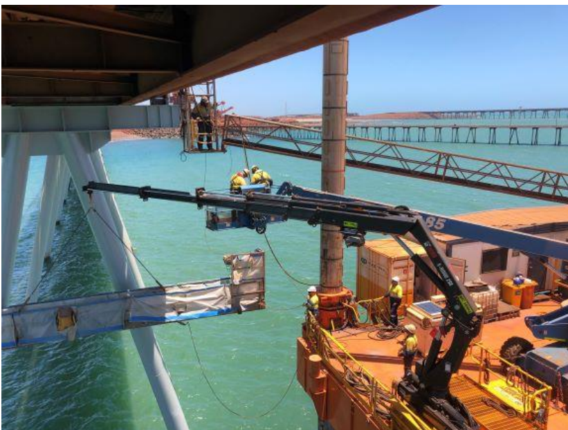
Pile painting with twin level horseshoe platforms + twin modular flatpack walkways along headstocks + ladder access to deck level
