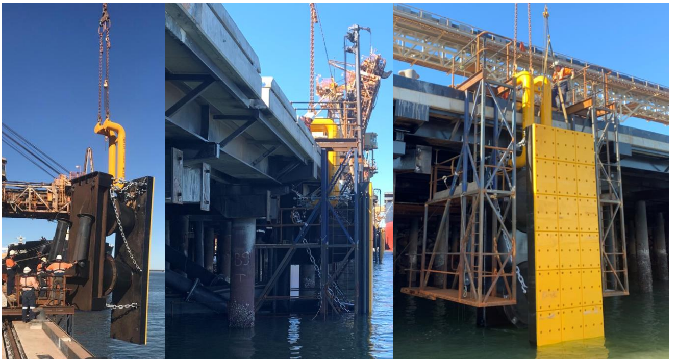
Installation of complete fender assembly with custom 25t C hook. Lift, rotate and install under edge of the wharf including scaffold access for brace installation.
