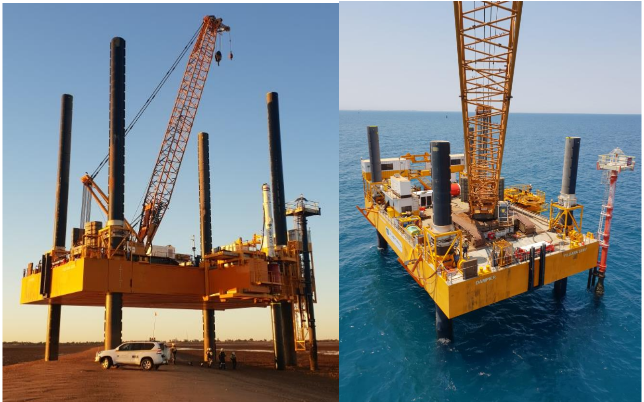
400t jackup on the tidal flat and offshore
